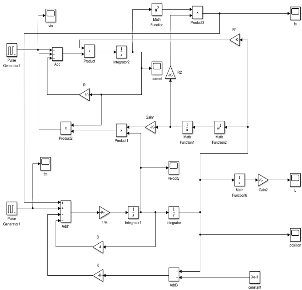
Simulation 2: Free-moving magnet simulation
