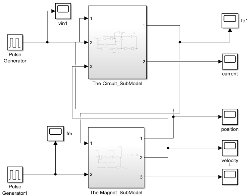
Simulation 3: Sub-layer Version
