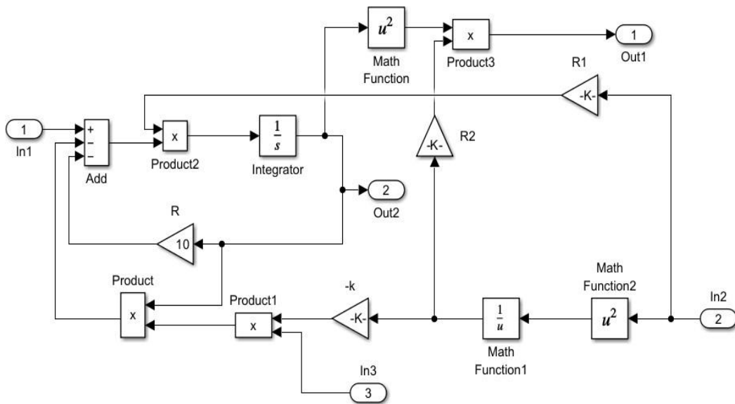
Simulation 3.1: The circuit_SubModel
